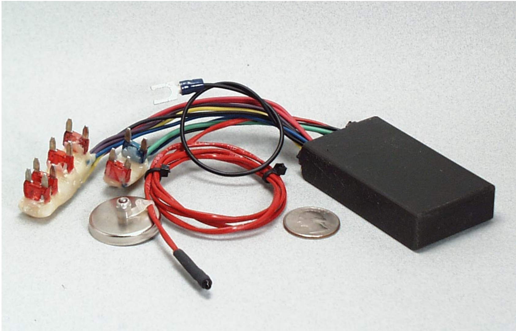
Fig 1a: First pre-production variation of the LightGenie for new and aftermarket vehicles of several platforms from different manufacturers when the case and the plugs are replaced by appropriate types. This particular unit in the figure is specifically made to be installed on a U.S. OEM or aftermarket Altima or Maxima in less than five minutes.
